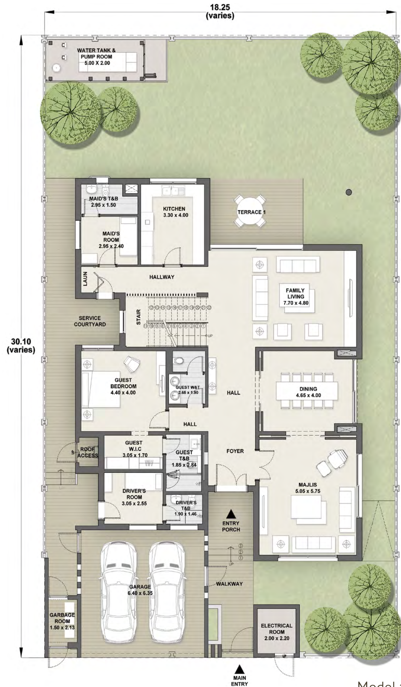
Ground Floor
